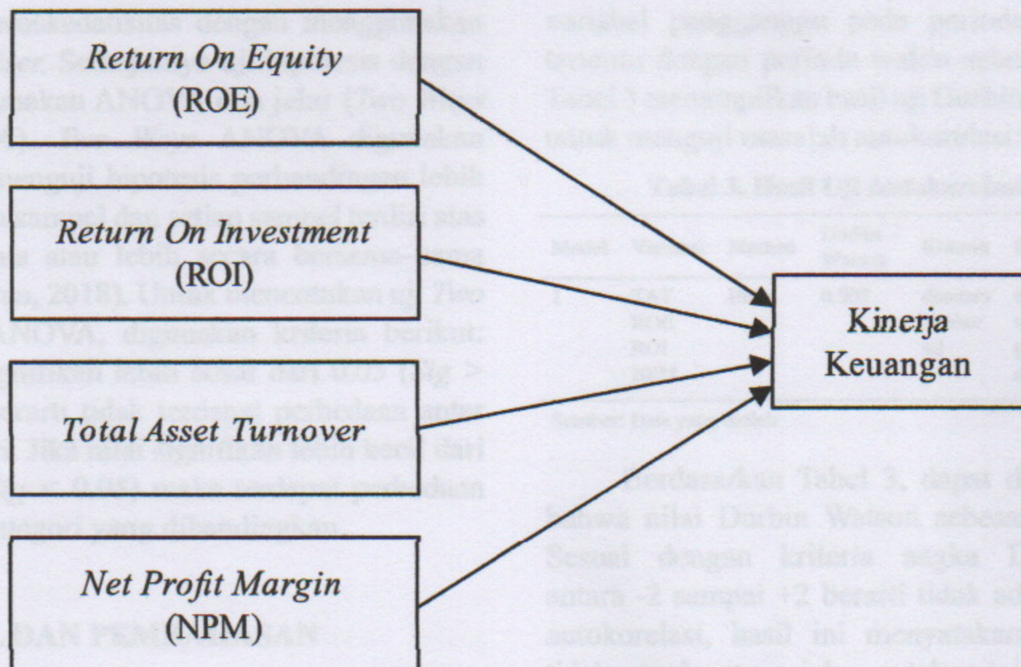
Gambar 1. Model Penelitian
